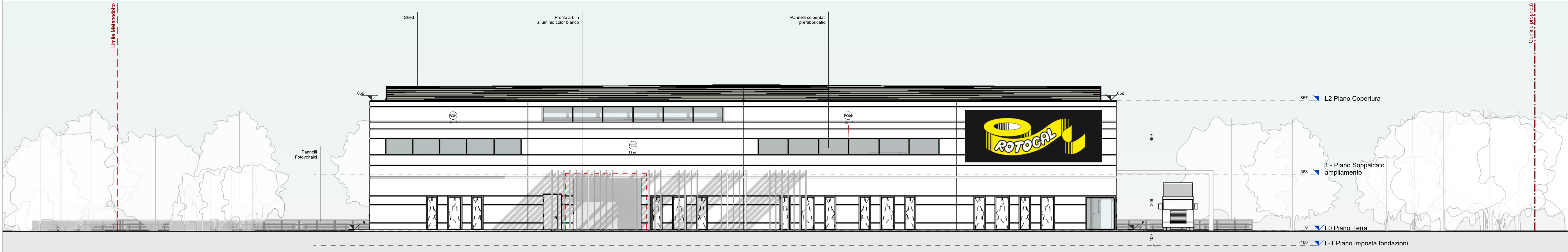
Prosp. Ovest 1 : 100
